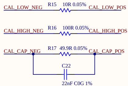
CALIBRATION LOADS
